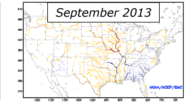
Daily streamflow anomaly
