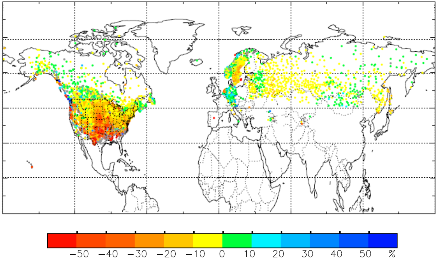
Comparison of POD between AFWA SNODEP and IMS Snow Cover
